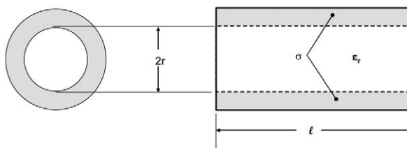
Figure 22: Circular waveguide dimensions and properties
